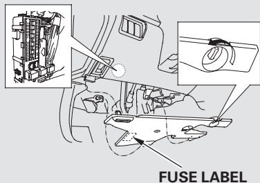
FUSE LABEL
