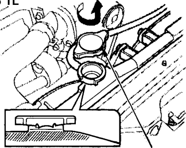
RADIATOR CAP
