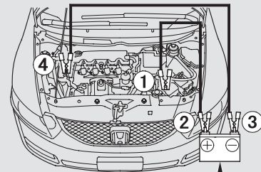
BOOSTER BATTERY
