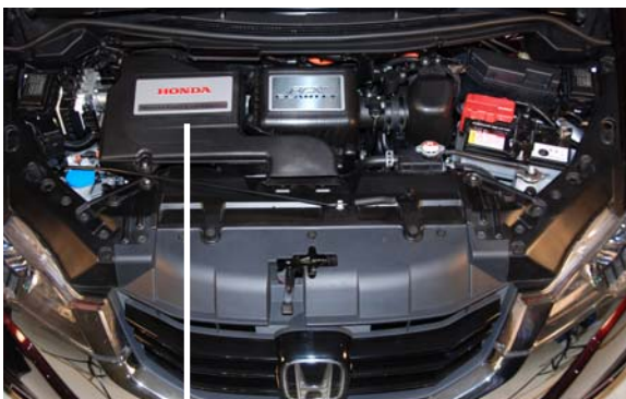
The Power Drive Unit (PDU) is located under other components and can be reached only by their removal.
