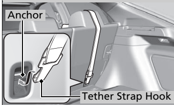
Straight Top Tether Type in Outer Position
