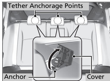
Straight Top Tether Type in Outer Position
