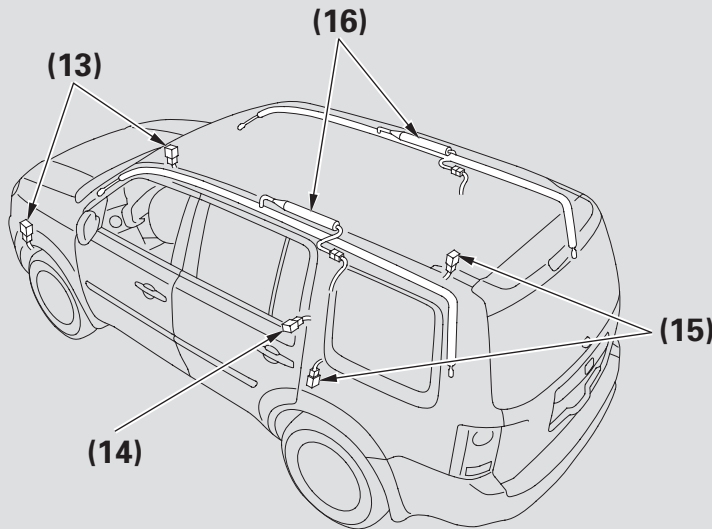
(13) Front Impact Sensors (14) Rear Safing Sensor (15) Side Impact Sensors (Second) (16) Side Curtain Airbags
